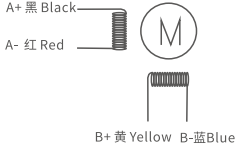
Motor Connctions
