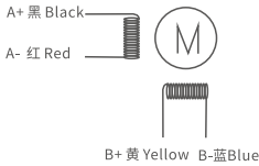
Motor Connctions
