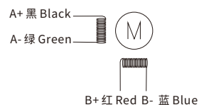
Motor Connections:
