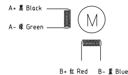
Motor Connections:
