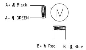
Motor Connections:
