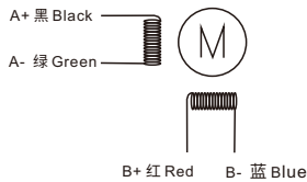
Motor Connections:
