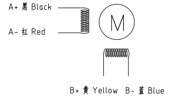
Motor Connections:
