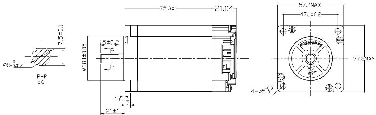
iCL57A-RS23
