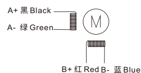
Motor Connections:
